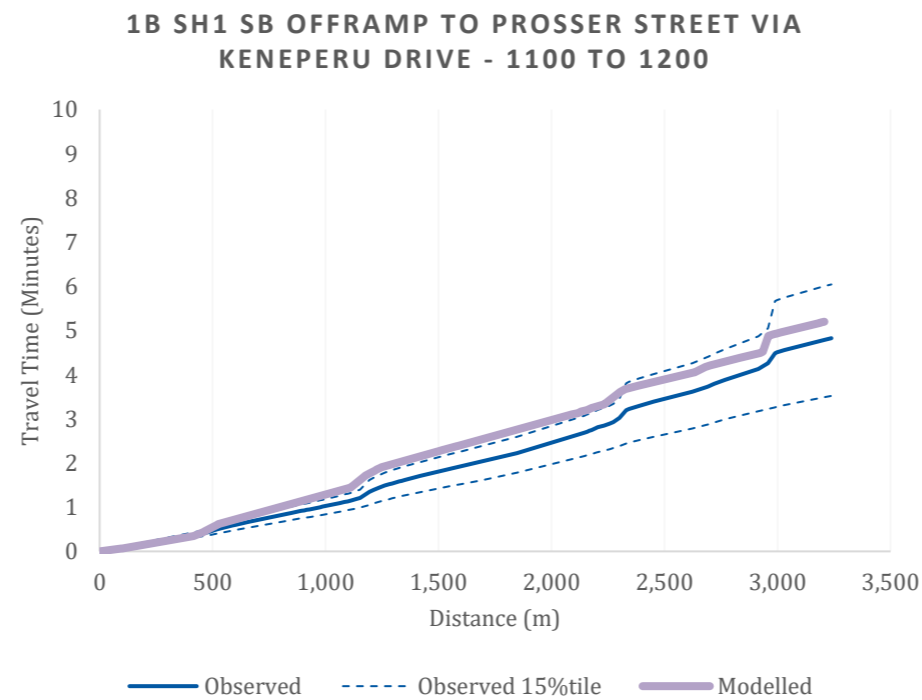
Figure D5: Journey time plot, R2: SH1 SB offramp to Prosser Street via Keneperu Drive inter peak hour
