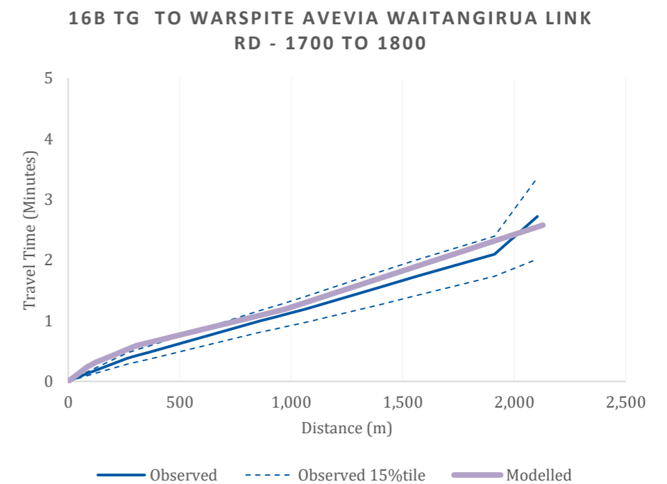
Figure D96: Journey time plot, R32: TG to Warspite Ave via Waitangirua Link Rd evening peak hour
