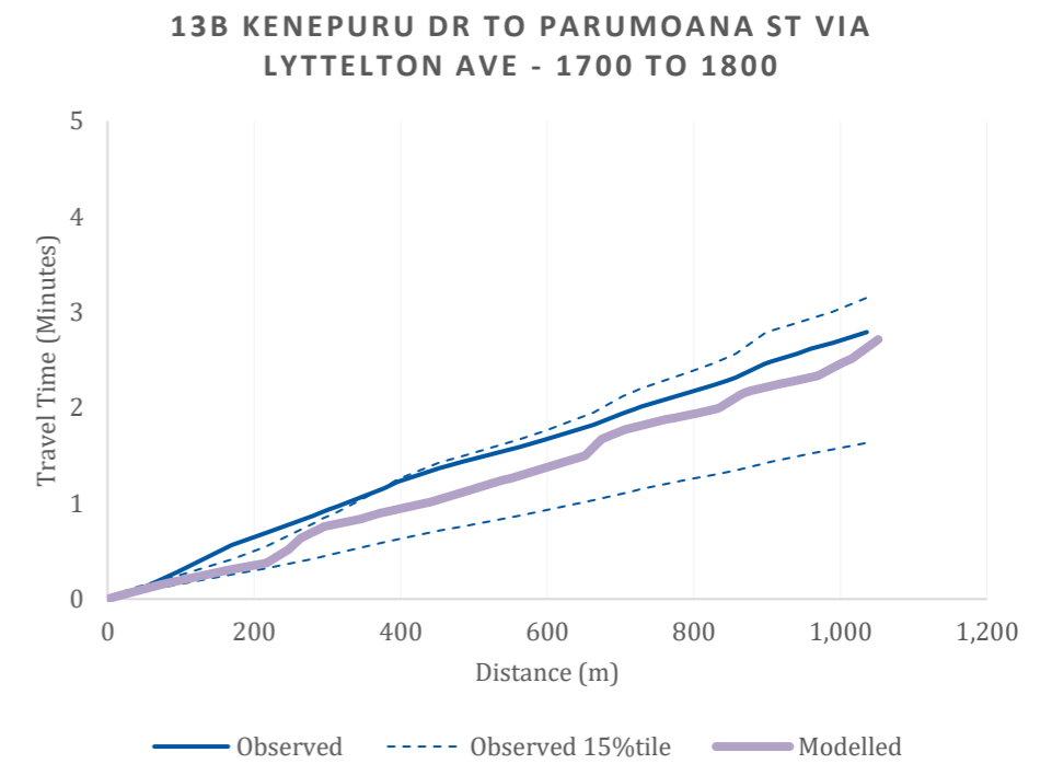
Figure D78: Journey time plot, R26: Kenepuru Dr to Parumoana St via Lyttelton Ave evening peak hour
