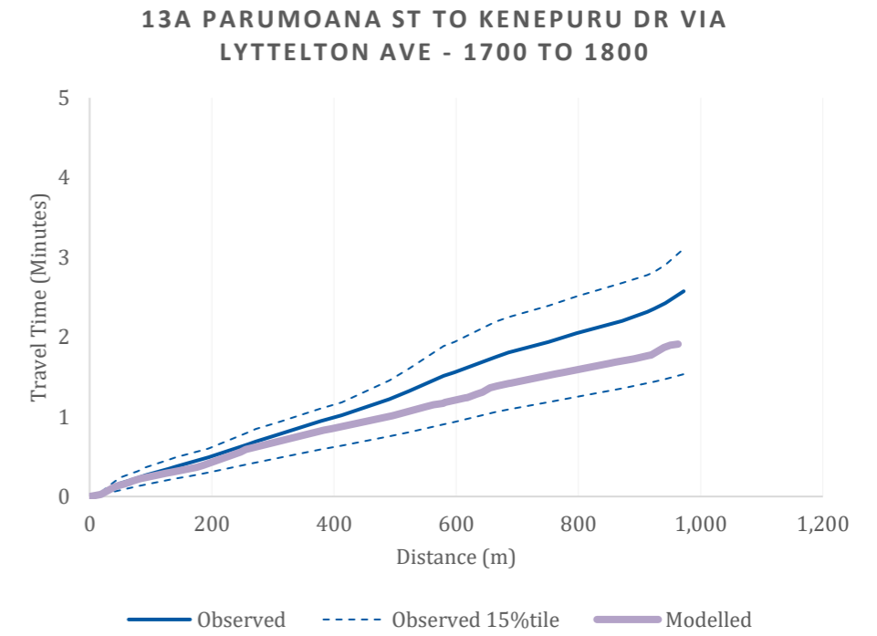
Figure D75: Journey time plot, R25: Parumoana St to Kenepuru Dr via Lyttelton Ave evening peak hour
