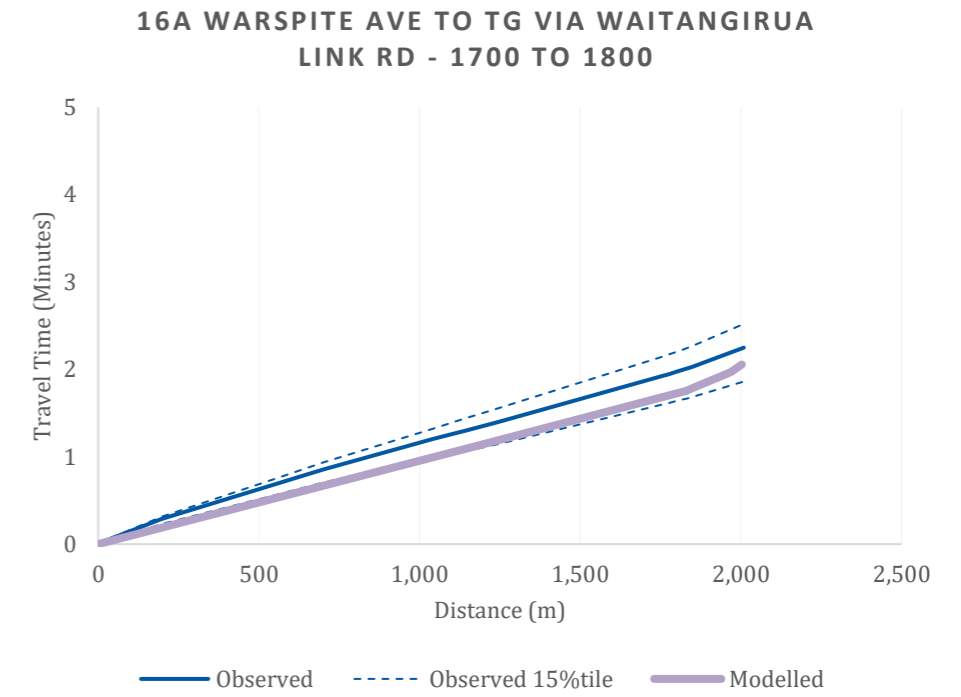
Figure D93: Journey time plot, R31: Warspite Ave to TG via Waitangirua Link Rd evening peak hour
