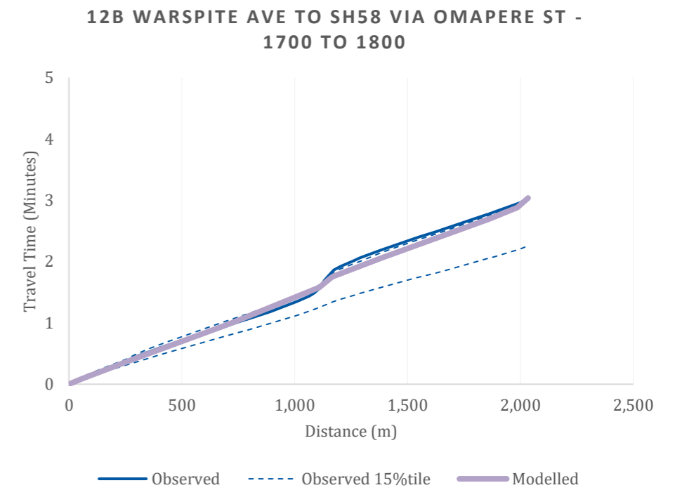
Figure D72: Journey time plot, R24: Warspite Ave to SH58 via Omapere St evening peak hour
